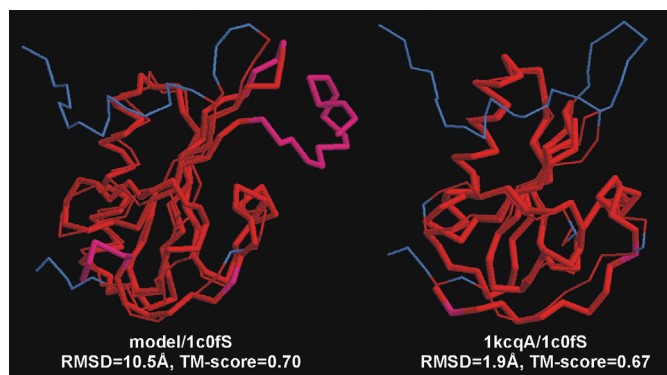
Figure 5. A comparison of a computer model generated by TASSER (8) and the closest PDB structure (template) found by TM-align. This is a typical example where the model has a much larger RMSD than the template because of the misoriented tails and loops. The thick backbones are the model or template and the thin ones the native structure of 1c0fS. The red residues are those residues where their distances are < 5 \text{ \AA} in the TM-score rotation matrix.
