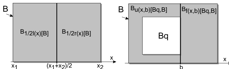
Fig. 2. Splitting operators
